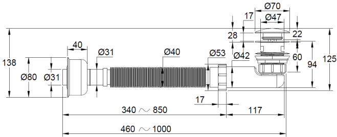
Siphon for bathtub # 700630
