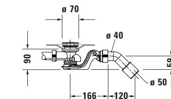
Siphon for bathtub # 700426
