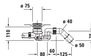
Siphon with base inlet for bathtub # 700426
