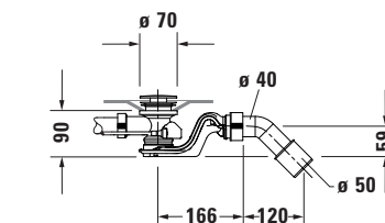
Siphon for bathtub # 700428
