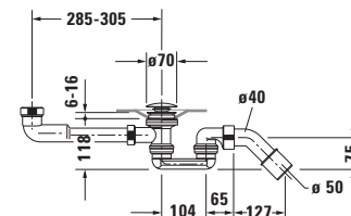
Siphon for bathtub # 700430
