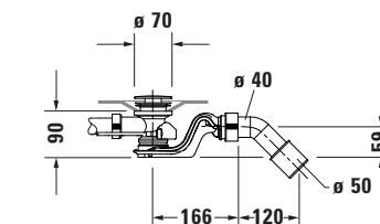
Siphon for bathtub # 700429
