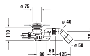
Siphon with base inlet for bathtub # 700429
