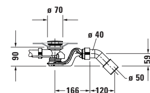
Siphon for whirltub # 760426
