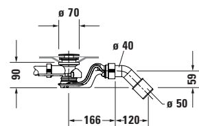
Siphon for whirltub # 760427
