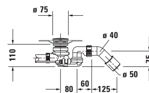
Siphon with base inlet for bathtub # 700428
