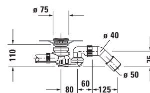
Siphon with base inlet for whirltub # 760428
