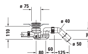
Siphon with base inlet for whirltub # 760426
