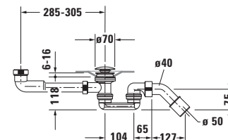
Siphon for bathtub # 700460
