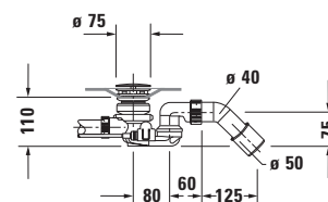
Siphon with base inlet for bathtub # 700427
