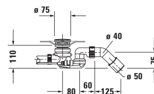
Siphon with base inlet for whirltub # 760427
