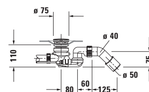
Siphon with base inlet for whirltub # 760429
