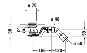
Siphon for whirltub # 760428
