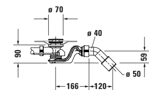
Siphon for whirltub # 760429
