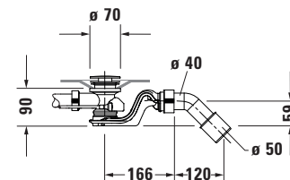
Siphon for bathtub # 700427
