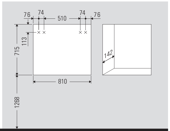
Cutout dimensions for built-in cabinets
